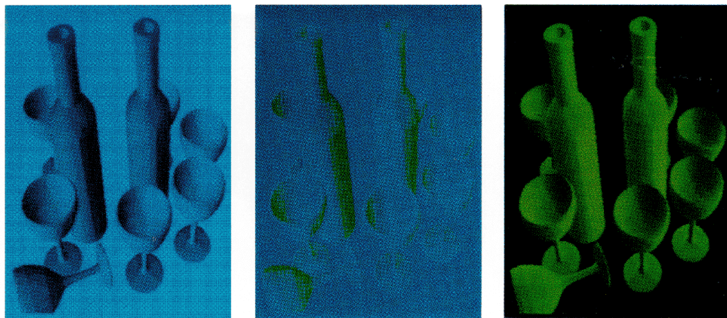
Fig. 7. Computer-generated images in which shape is generated by shading. In the middle image the two colors are equiluminant, and the three-dimensional shape is harder to discern than in the other two images, which have luminance-contrast.
