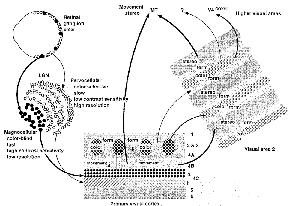
Fig. 4. Diagram of the functional segregation of the primate visual system. MT, middle temporal lobe; V4, visual area 4; LGN, lateral geniculate body.
